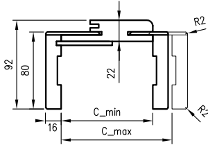
ORB cross-section 075
