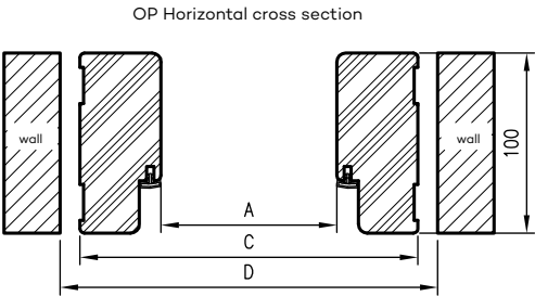
required height of wall passage 2089 mm (2095 mm for glass doors)
