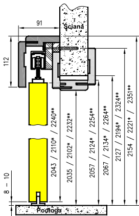
NS - vertical cross-section for tunnel with 63 mm architrave NT - vertical cross-section for tunnel with 80 mm architrave
