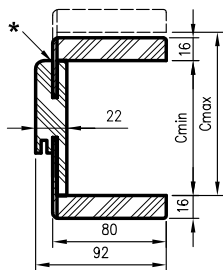
cross-section of vertical beam
