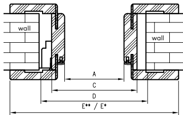
OR/ORC horizontal cross-section
