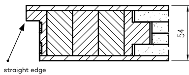
Anti-burglary and fire-resistant door leaf NEFRYT RC2/RC3 EI-30
