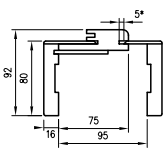
ORB cross-section 075
