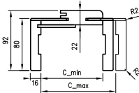
ORB cross-section 075
