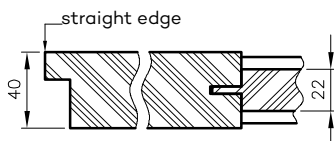
Horizontal cross-section of Nestor
