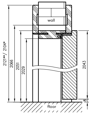
vertical cross-section of glass doors with ORC (adjustable door frame for glass doors)
