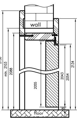
vertical cross-section of ORO
