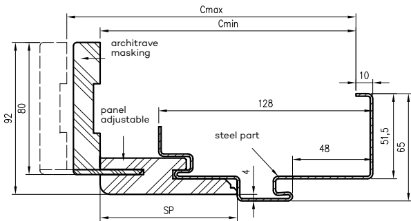
OSH door frame profile
