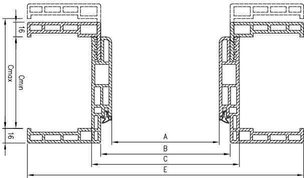
Width of the door frame of a single-leaf rebated door
