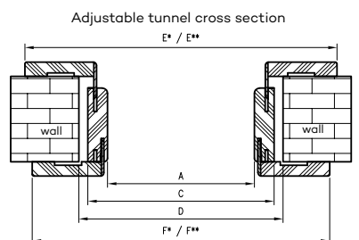
TUN cross-section with T63
