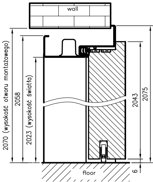
Olimp EI60 dimensions for single leaf doors
