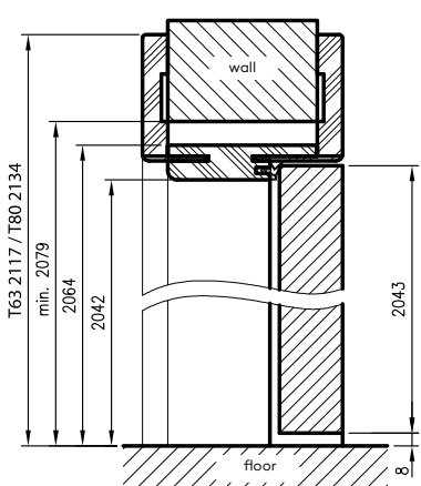
Vertical section of the door non-rebated door leaf
