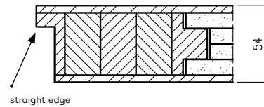
NEFRYT RC2/RC3 anti-burglary door leaf
