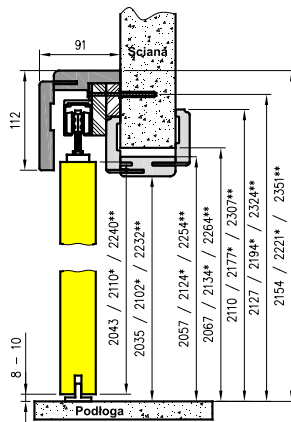
NS - vertical cross-section for tunnel with 63 mm architrave NT - vertical cross-section for tunnel with 80 mm architrave
