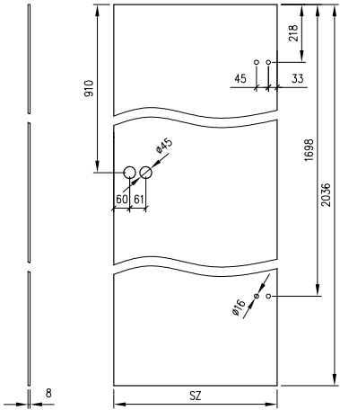
glass door leaf a) swing
