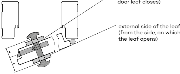
fig. selection of cylinder insert dimension with door knob
